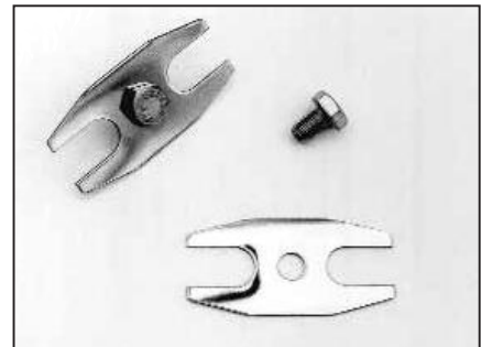
PI injector keeper plate 149308 and stainless steel hexagon screws. Also TR5 and TR6, set of 3. £7.05
